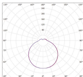
DAISY NAL-S 24W NW GXDS164
