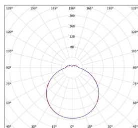
DAISY NAL-S 12W NW GXDS134
